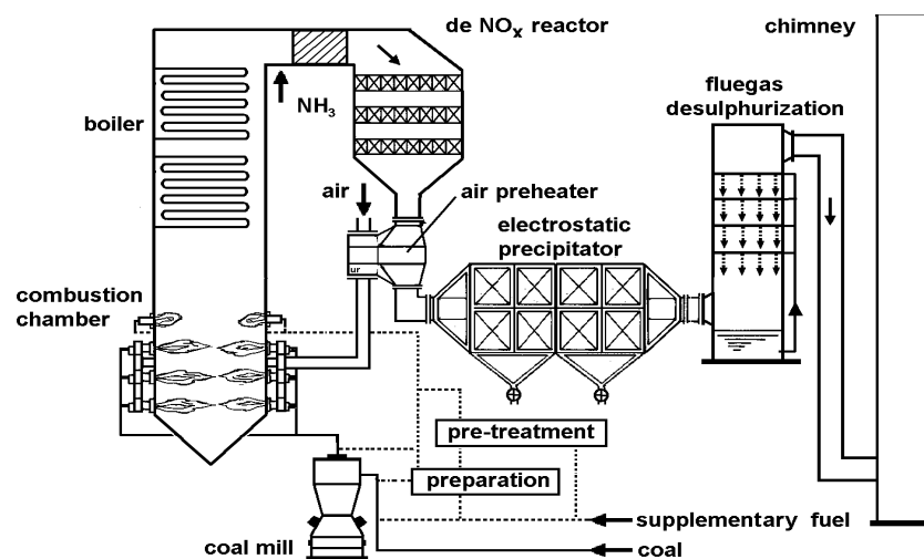
Fig. 2: Schematic diagram of a typical pulverized-coal-fired power plant with flue gas treatment system
